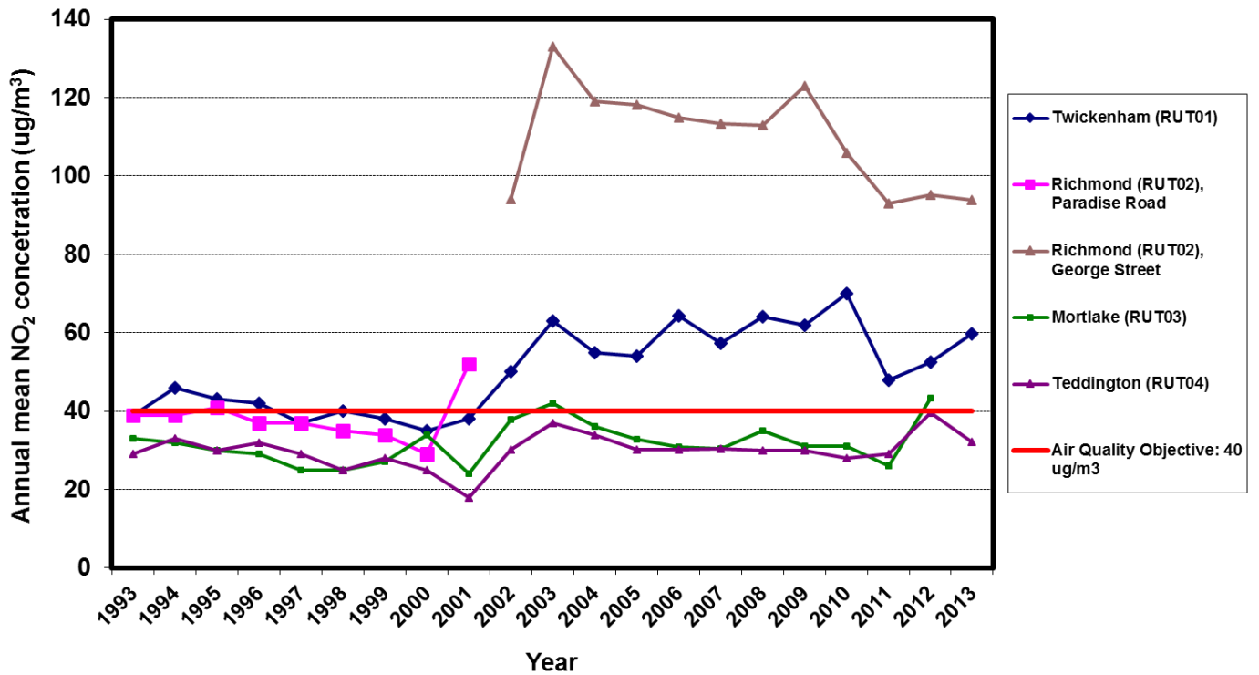
Figure 3: Annual mean NO 2 from 1993 to 2013 (Chart of Table 11 data, bias corrected from 2002 onwards, because there was no bias correction data available for the earlier years). Note: the Richmond site moved from the police station rear courtyard on Lewis Road to George Street in July 2001. The higher concentrations from 2002 demonstrate the impact of the much heavier local traffic movements at the new site. In 3 rd January 2012 site RuT 03, Alexandra Hall, Mortlake was closed and RuT 04 moved from the side to the front of 4 Waldegrave Road, Teddington
