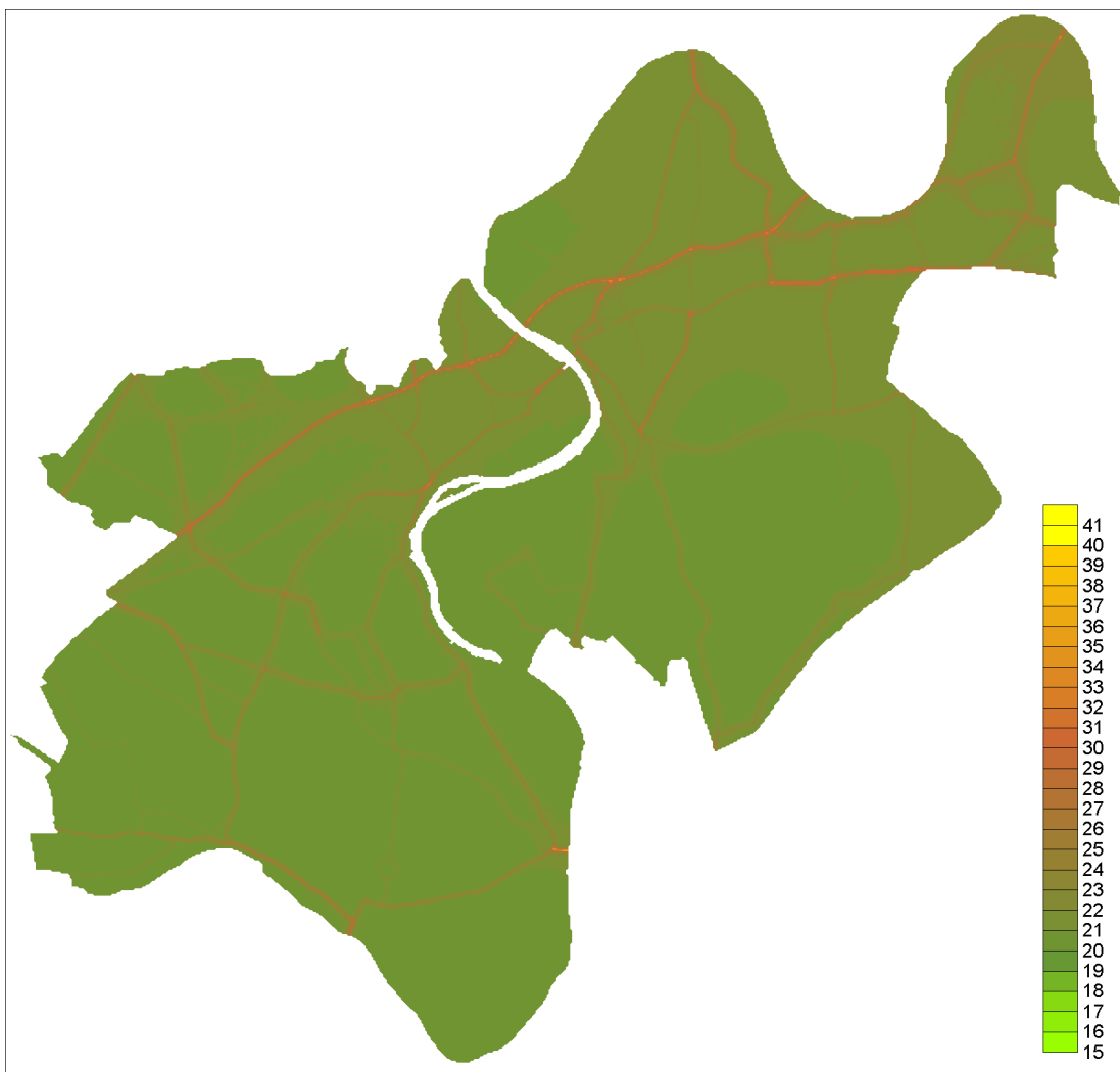
Figure 2: Modelled PM 10 concentrations in LBRuT for 2015. (Modelled by ERG from 2010 data)
