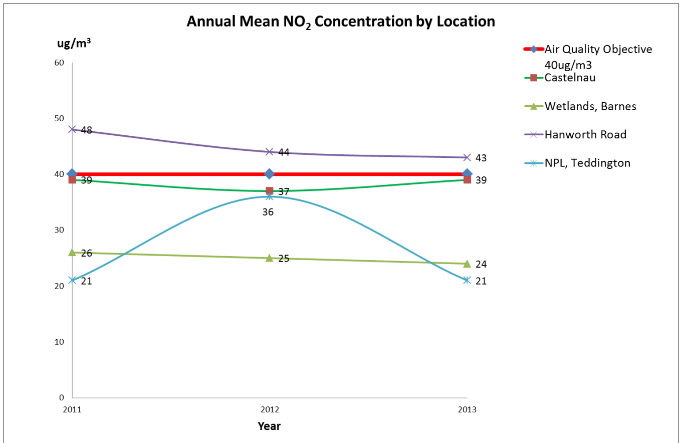
Figure 7 Trends in Annual Mean Nitrogen Dioxide Concentration Measured at Automatic Monitoring Sites (graph includes data from Table 14a)
