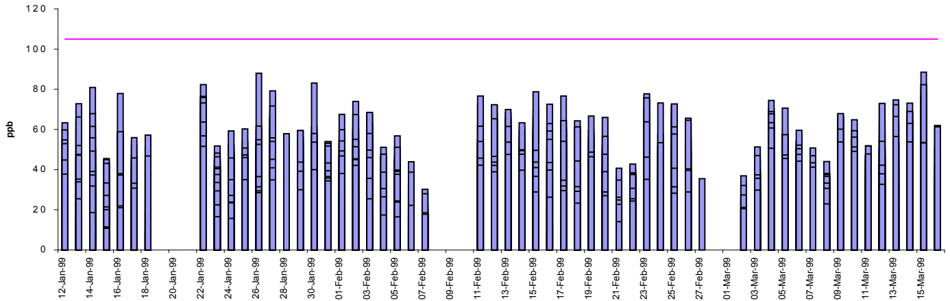
Sulphur Dioxide (SO 2 ) 15 min mean moderate up to 100ppb
