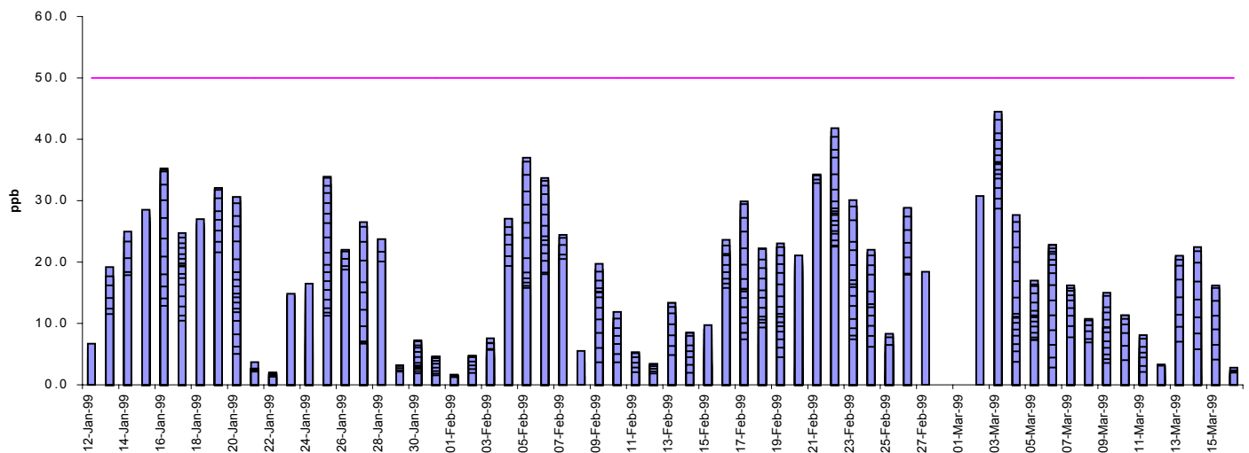
Ozone (O 3 ) Running 8 Hour Mean Low up to 50ppb
