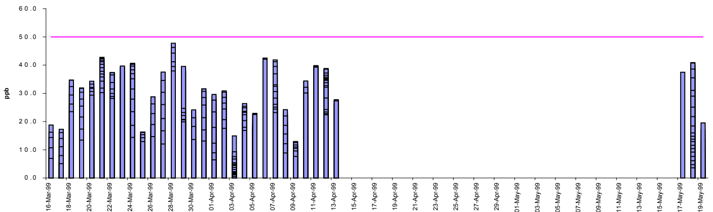
Ozone (O 3 ) Running 8 Hour Mean Low up to 50ppb
