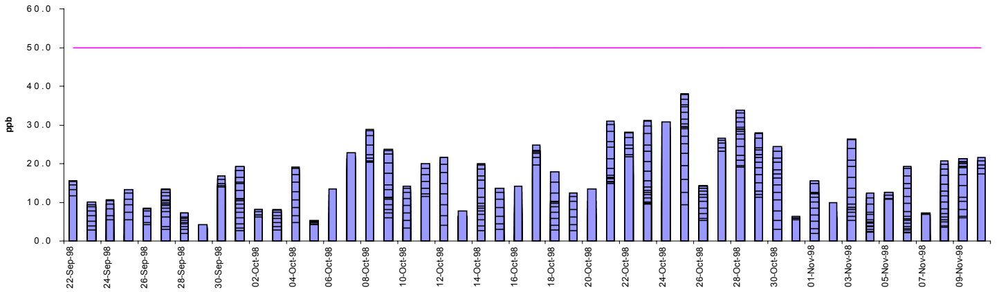
Sulphur Dioxide (SO 2 ) 15 min mean moderate up to 100ppb
