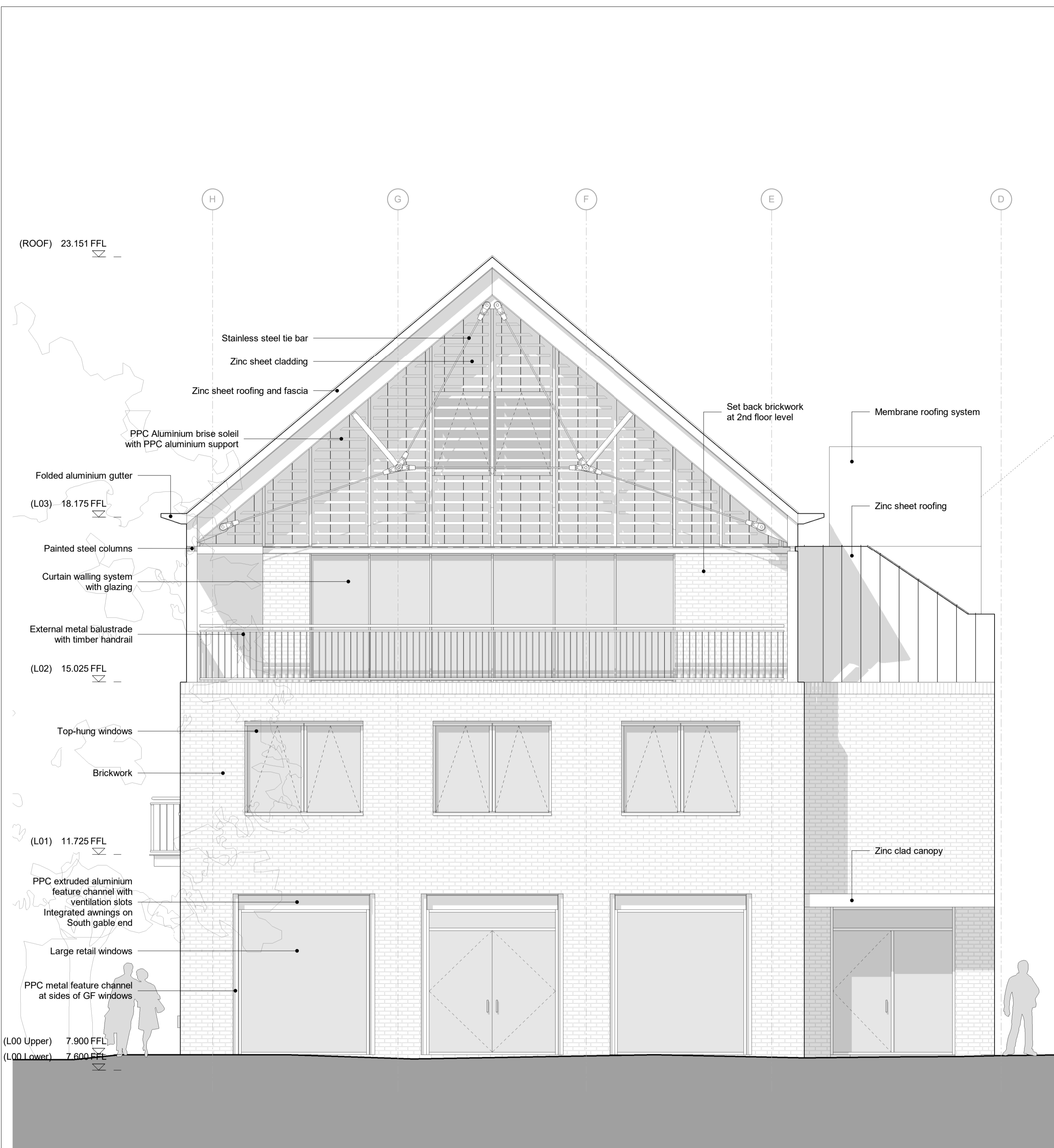
1 Water Lane - Gable End Typical Bay 2695 1:50
