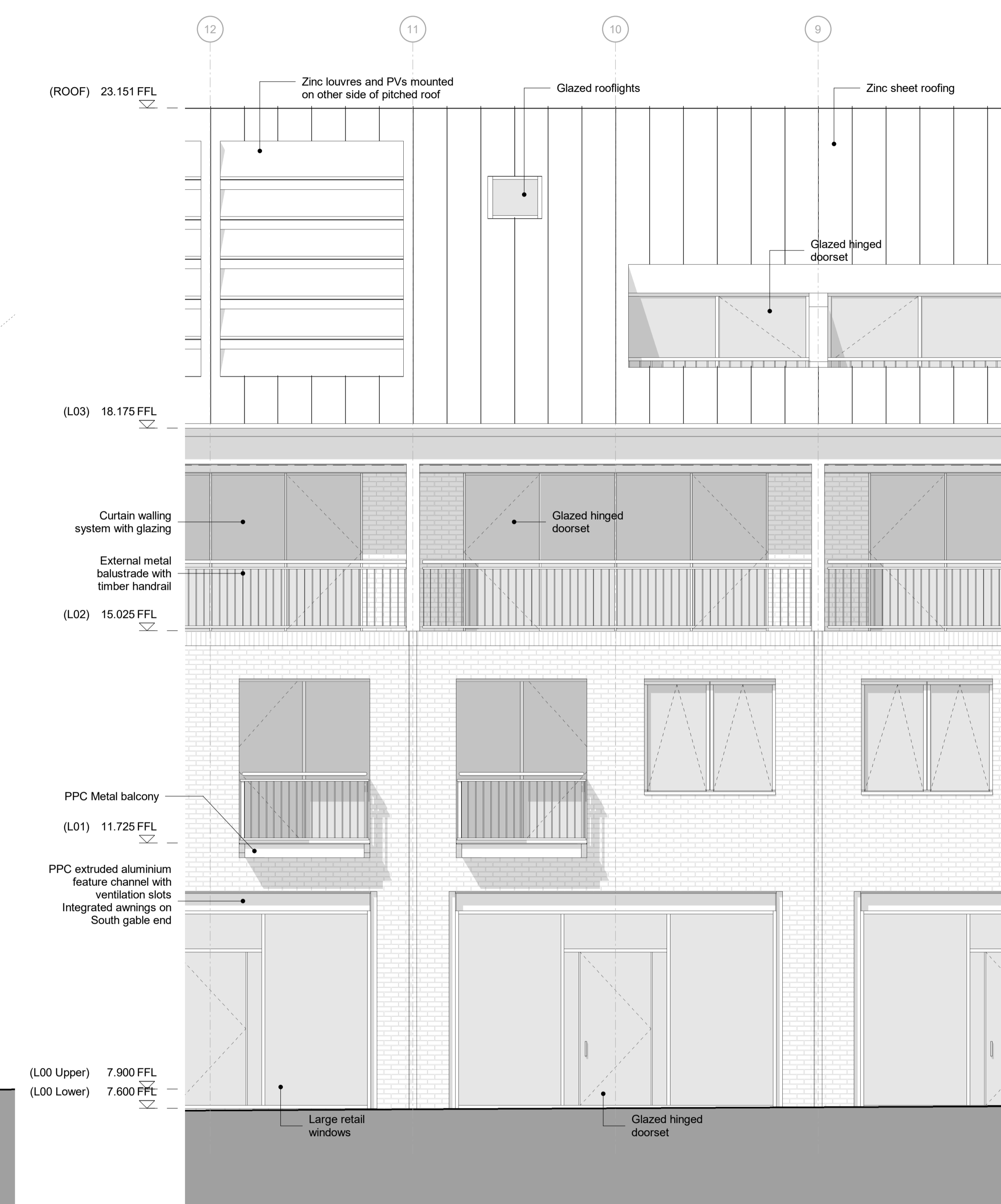
2 Water Lane - Water Lane Typical Bay 2695 1:50
