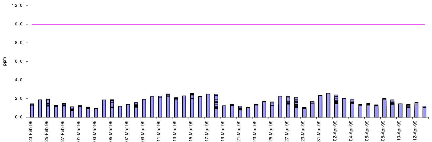
Carbon Monoxide (CO) Running 8 Hour Mean Limit=10ppm
