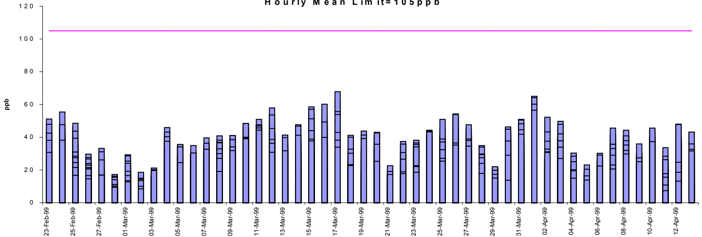
Nitrogen Dioxide (NO 2 ) Hourly Mean Limit=105ppb
